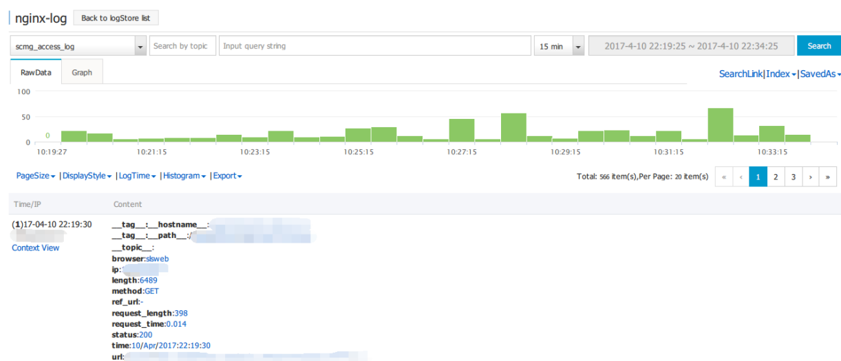
Figure 3-20: Preview
