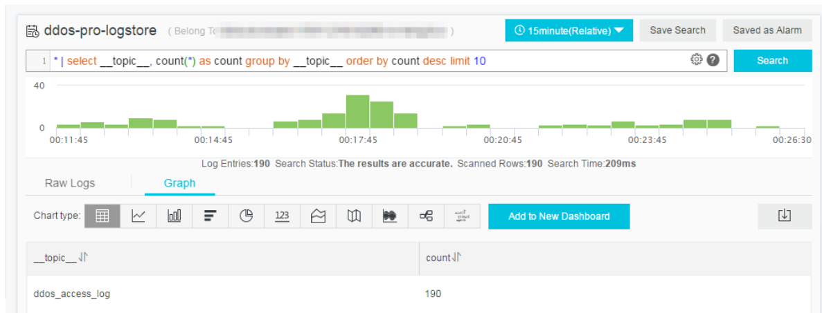
Figure 4-10: Statistic chart
