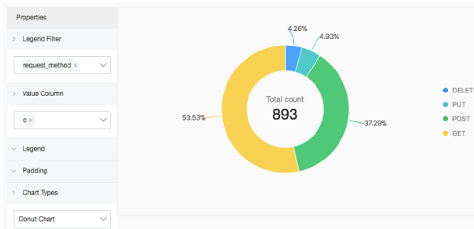
Figure 7-17: Cycle graph
