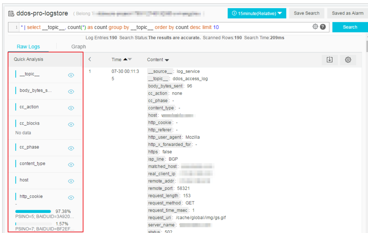
Figure 4-11: Quick analysis
