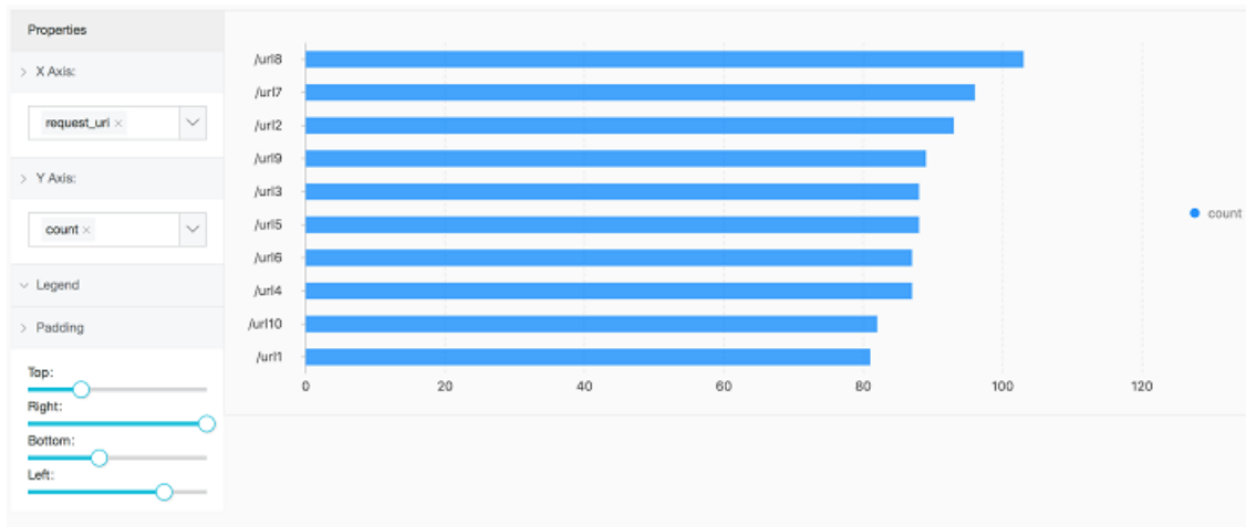
Figure 7-15: Simple bar chart
