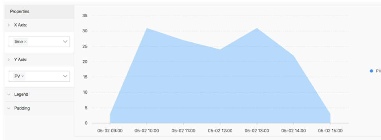
Figure 7-19: Simple area chart
