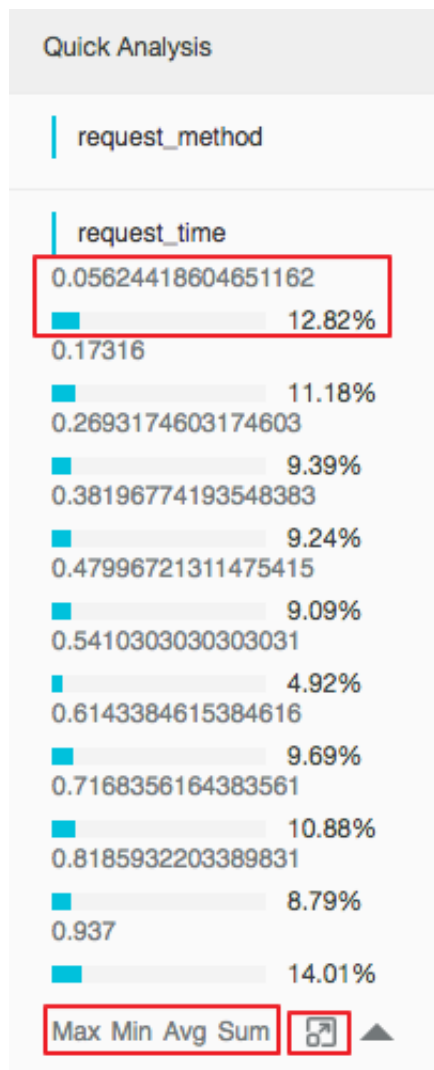
Figure 6-8: Request Distribution
