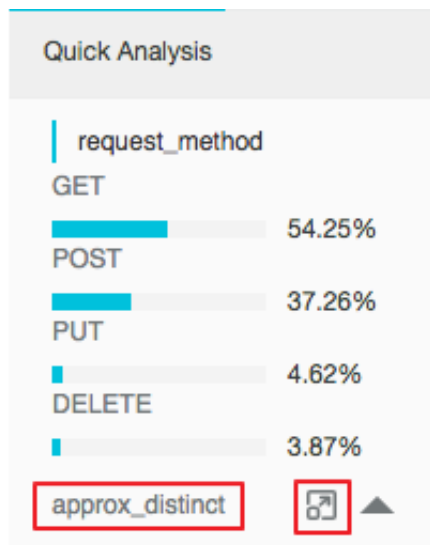
Figure 6-7: Group statistics
