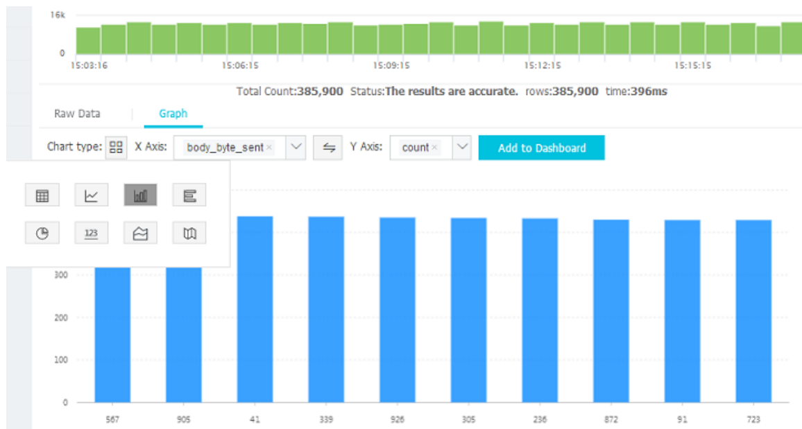
Figure 6-10: Dashboard
