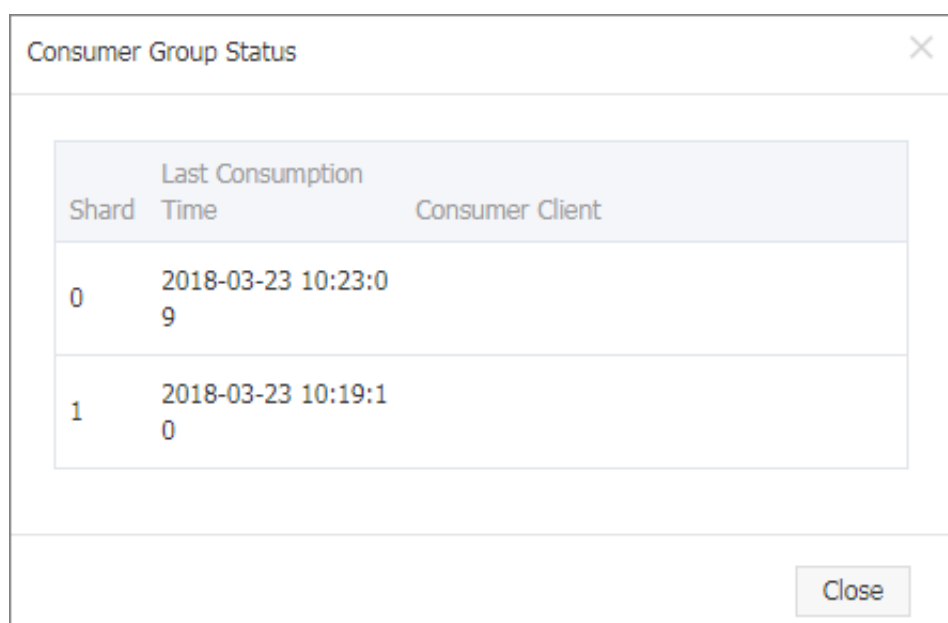
Figure 9-3: Consumption status
