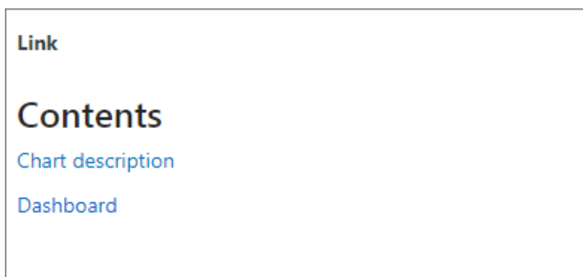
Figure 7-4: Link preview
