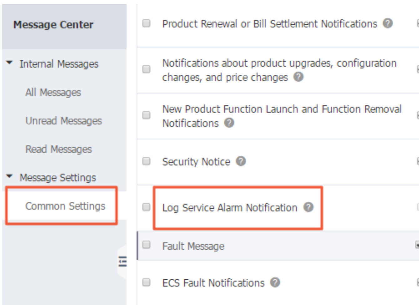
Figure 8-7: Common Settings
