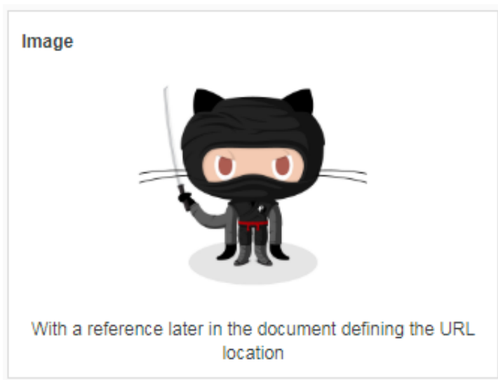
Figure 7-5: Image preview
