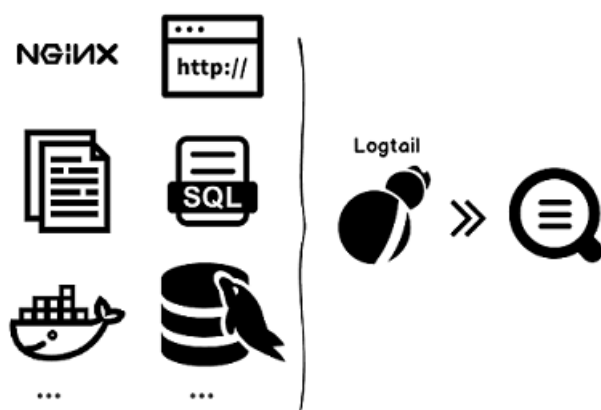
Figure 3-1: Function advantages
