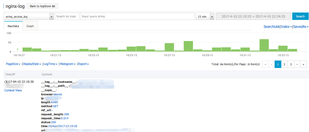
Figure 6-4: Query log
