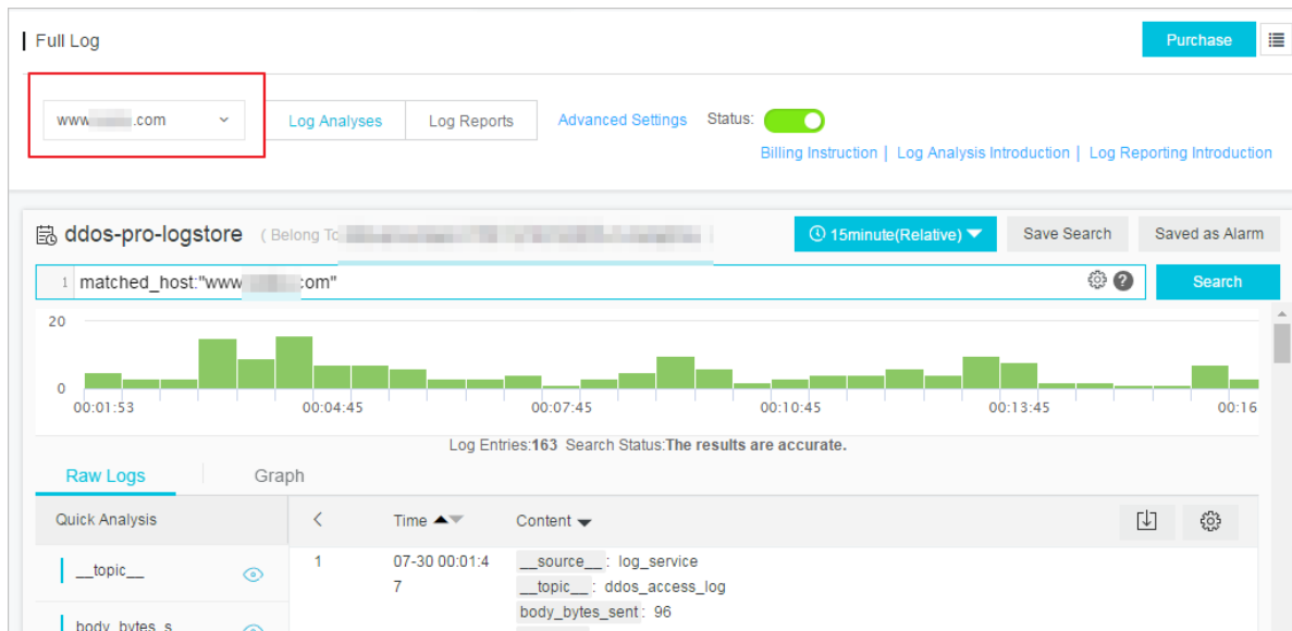
Figure 4-6: Log analysis
