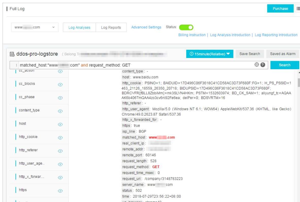
Figure 4-9: Raw logs
