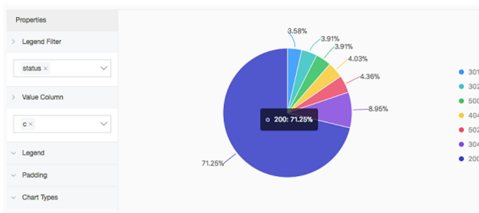
Figure 7-16: Pie chart
