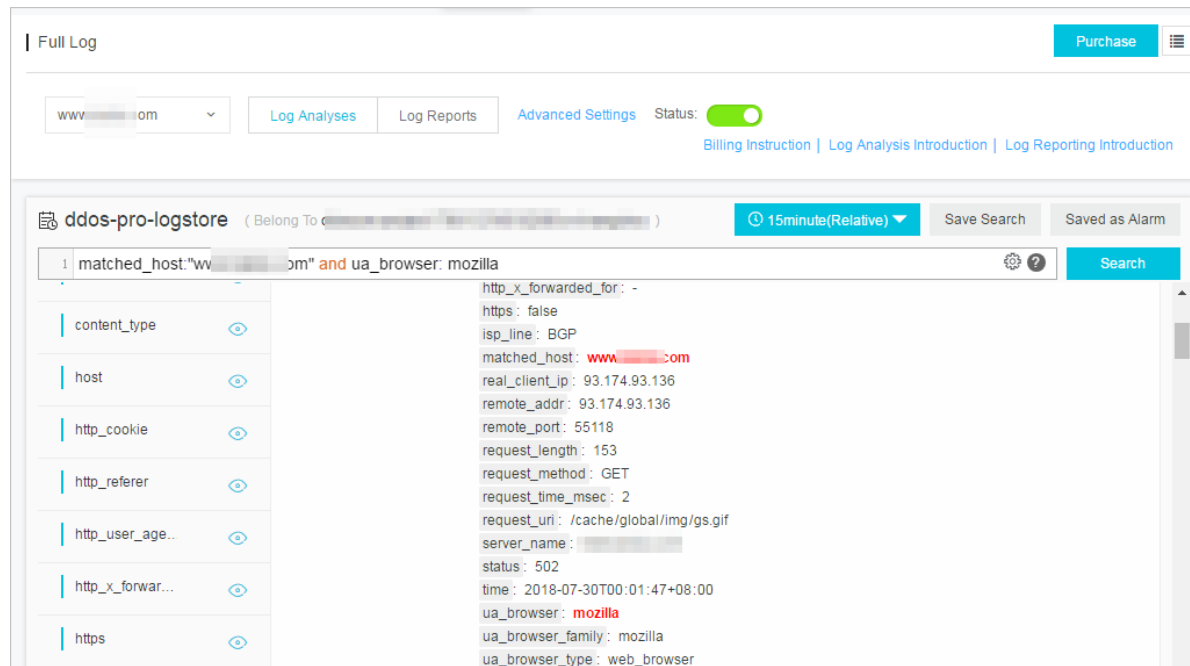
Figure 4-7: Log query
