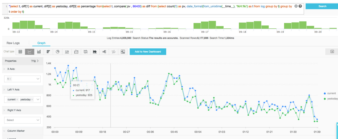
Figure 6-13: Line chart
