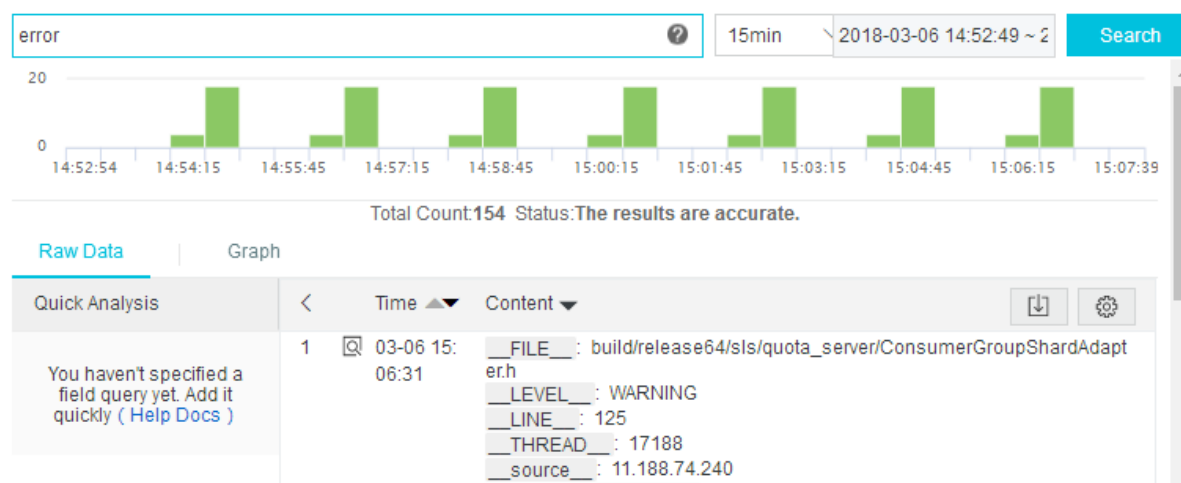
Figure 8-1: Raw log
