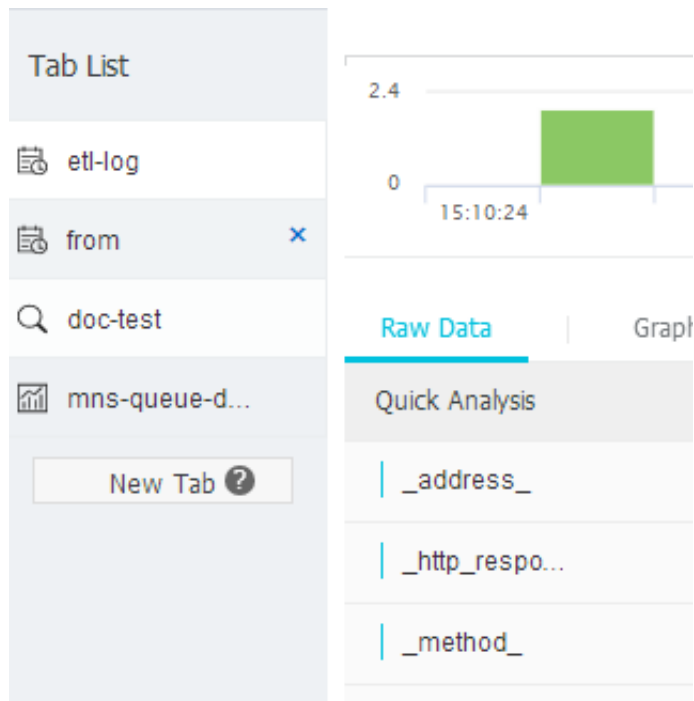
Figure 6-11: Tag
