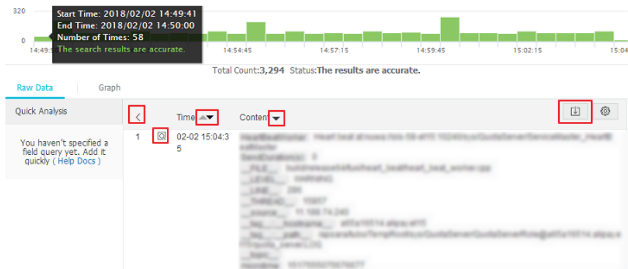
Figure 6-9: Raw logs
