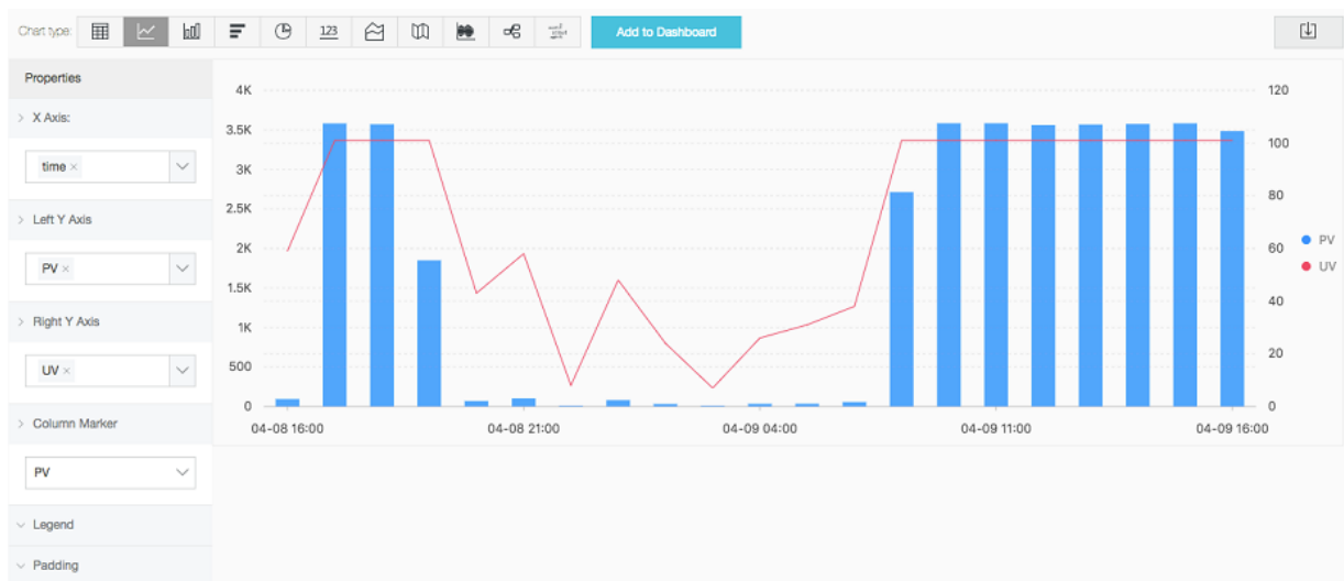
Figure 7-12: Line chart with both left Y axis and right Y axis
