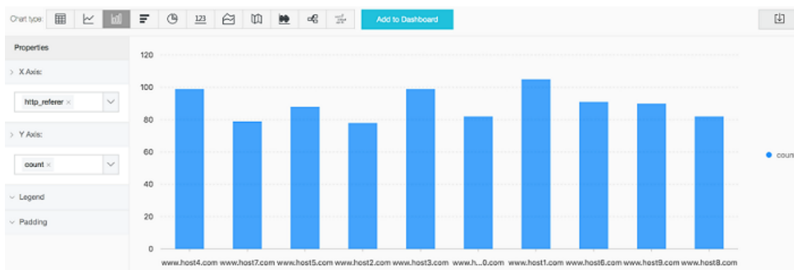
Figure 7-13: Simple column chart
