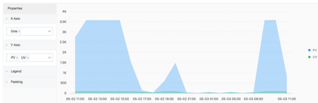
Figure 7-20: Stacked area chart
