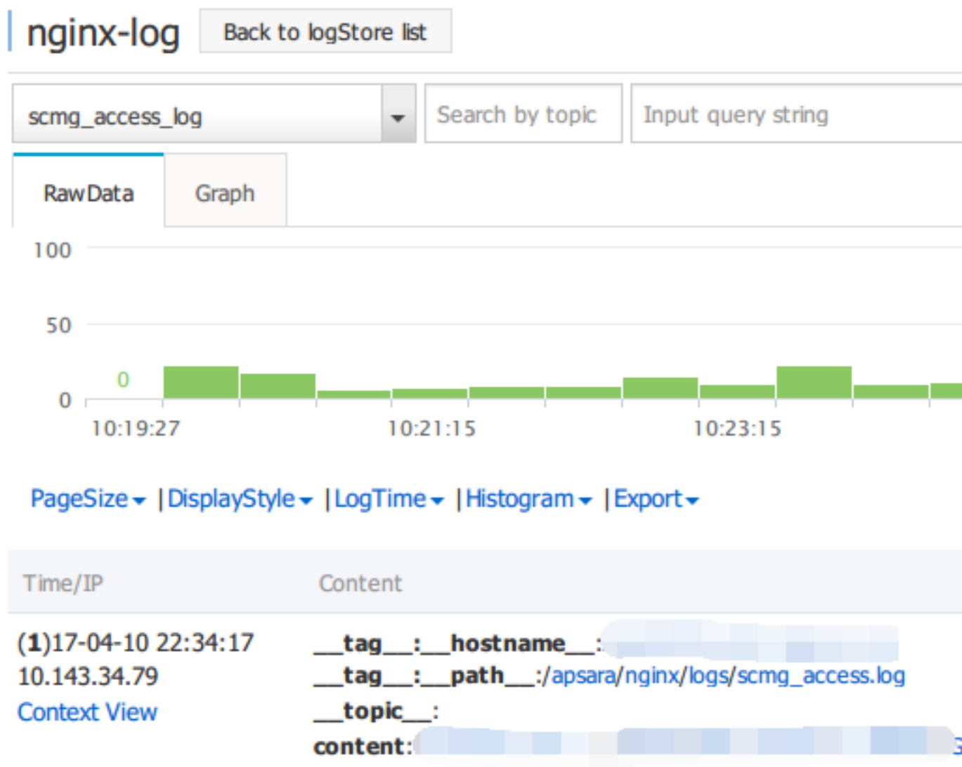
Figure 3-19: Preview
