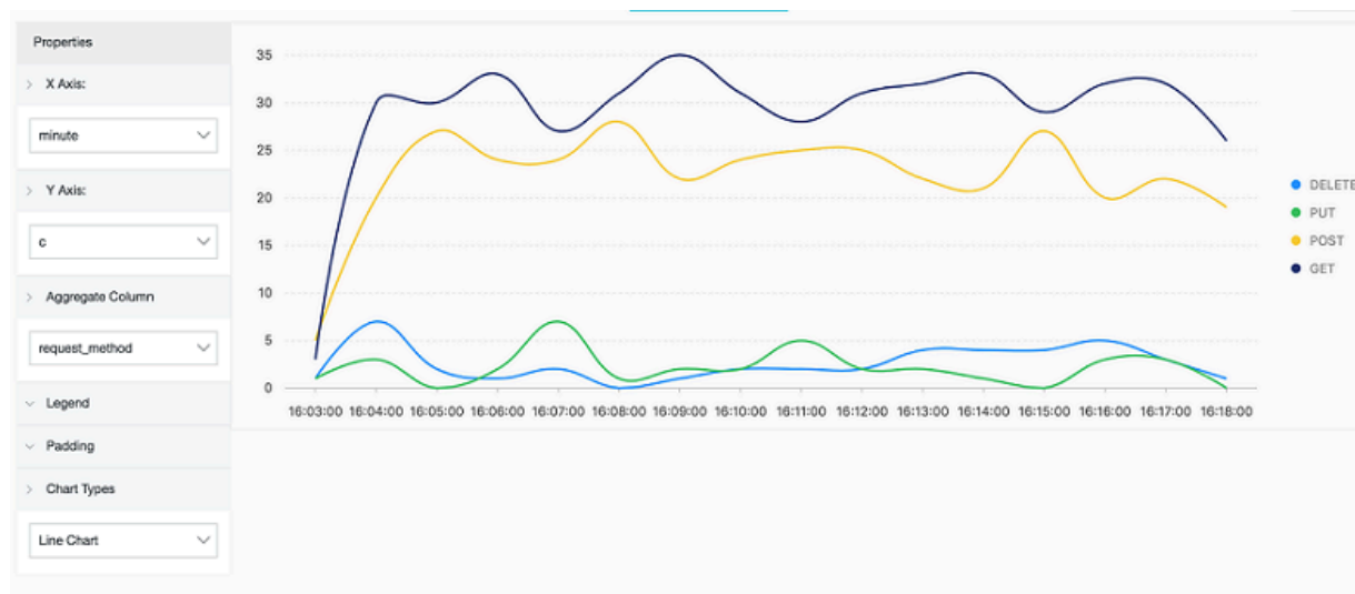
Figure 7-15: Flow chart
