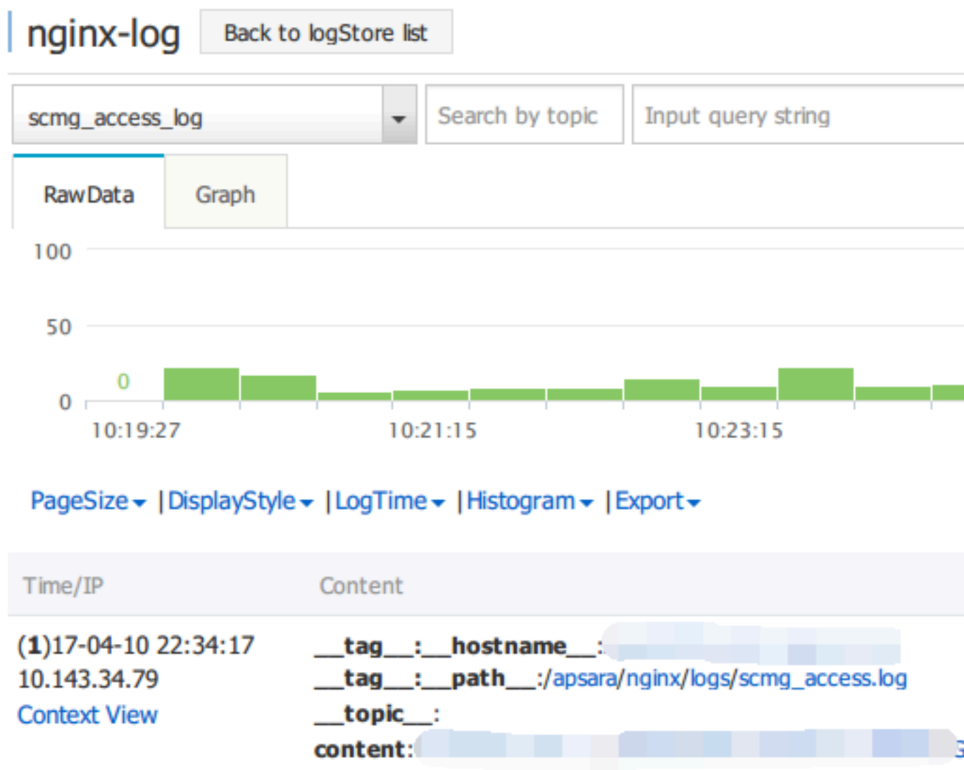
Figure 3-17: Preview
