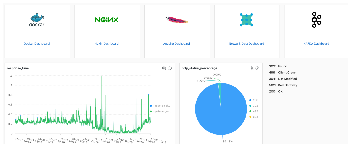
Figure 7-16: Scenarios
