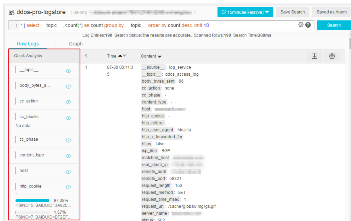
Figure 4-11: Quick analysis
