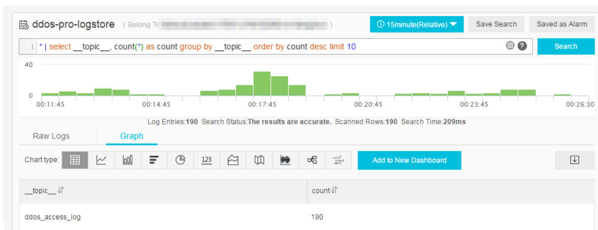
Figure 4-10: Statistic chart
