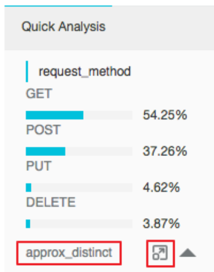
Figure 6-6: Group statistics
