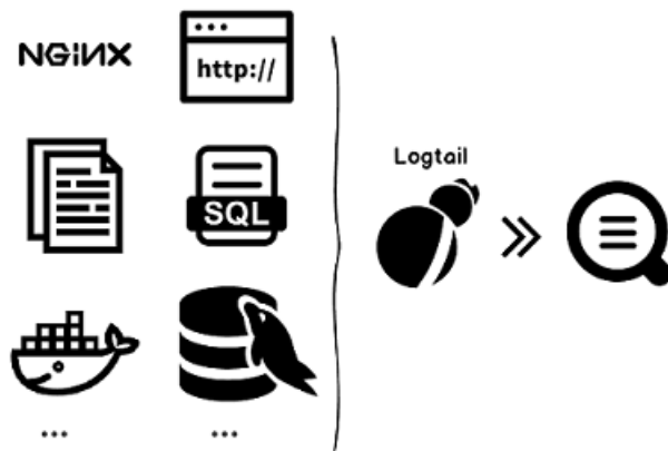
Figure 3-1: Function advantages
