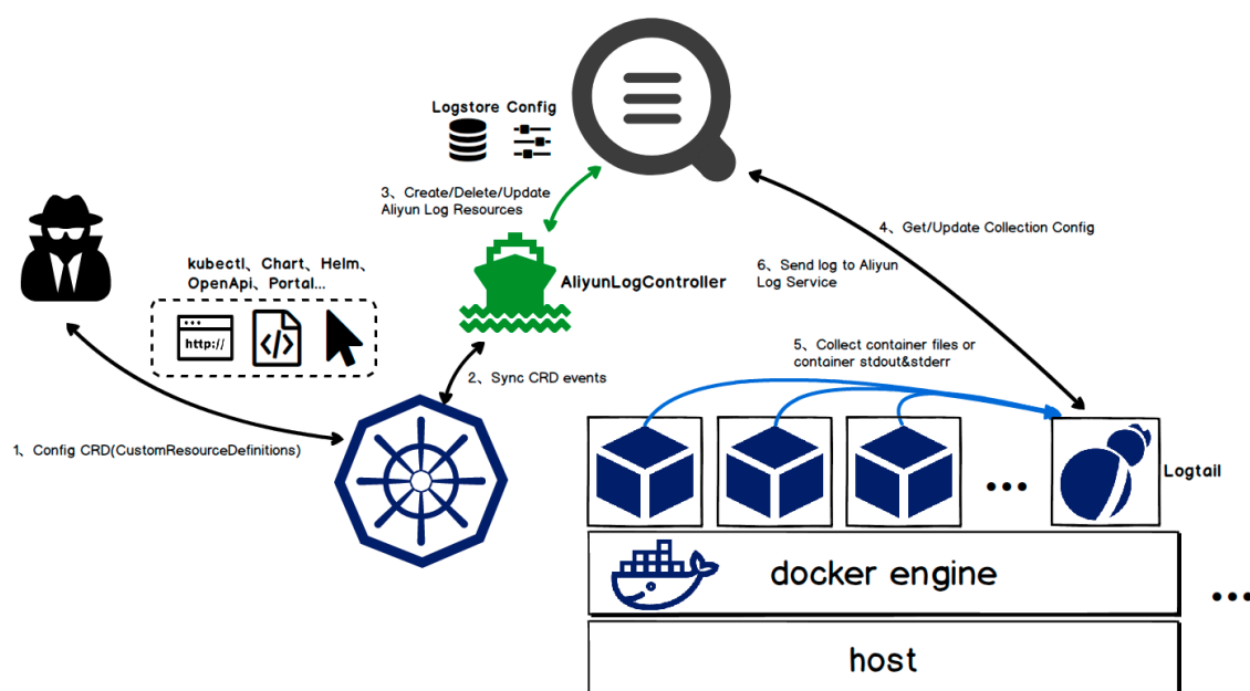
Figure 3-29: Implementation principles
