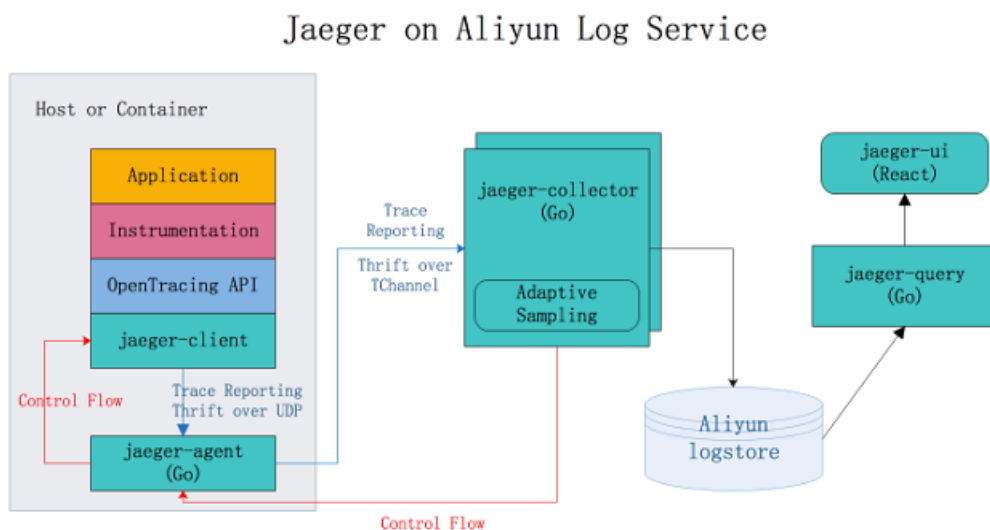
Figure 7-30: Jaeger
