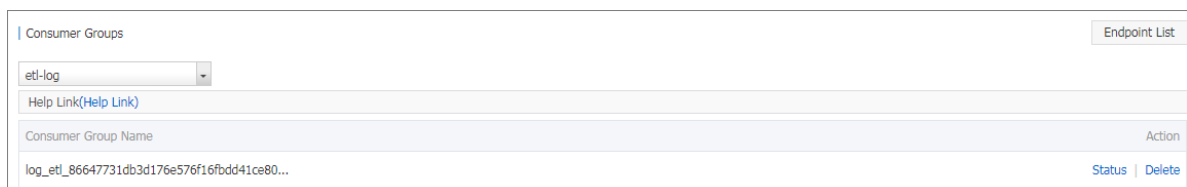
Figure 9-2: Consumer
