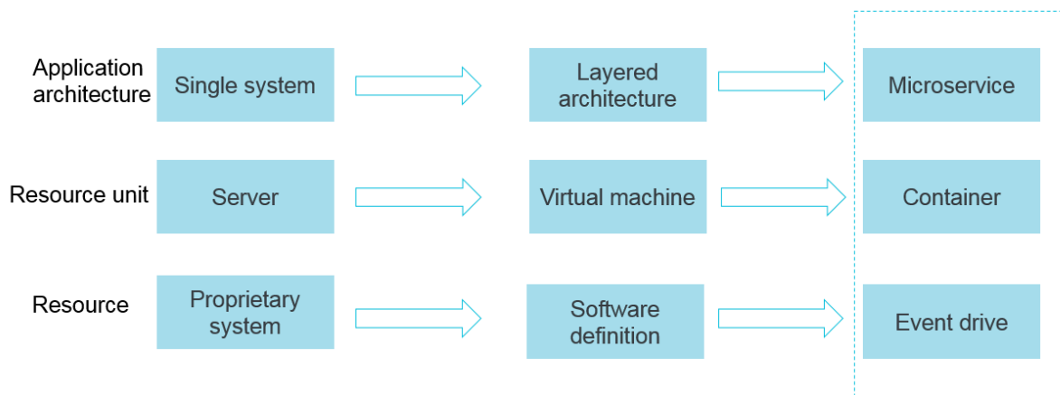
Figure 7-25: Architectural Evolution
