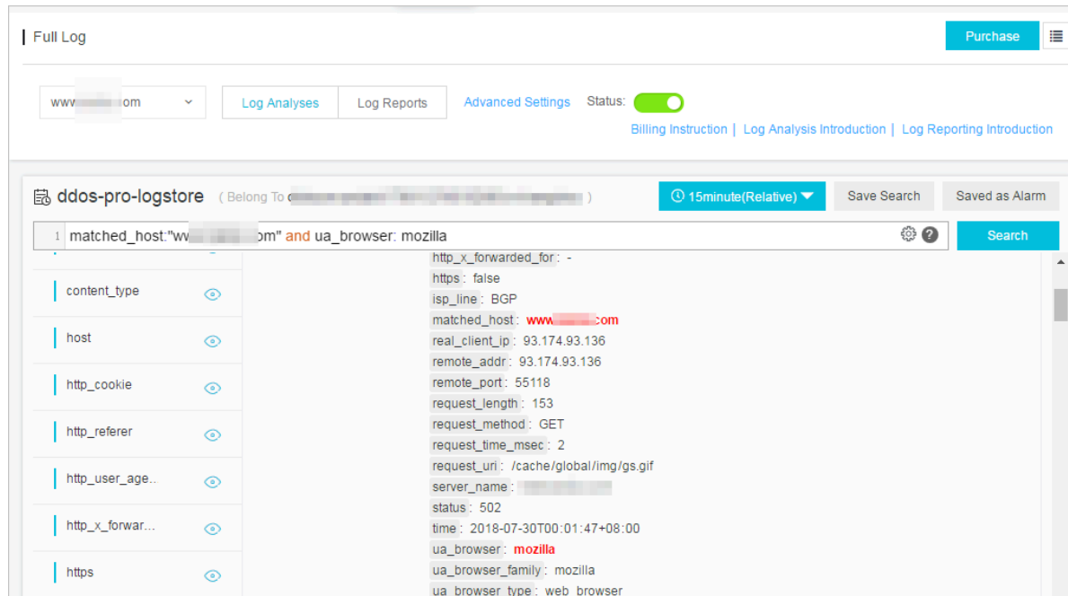
Figure 4-7: Log query
