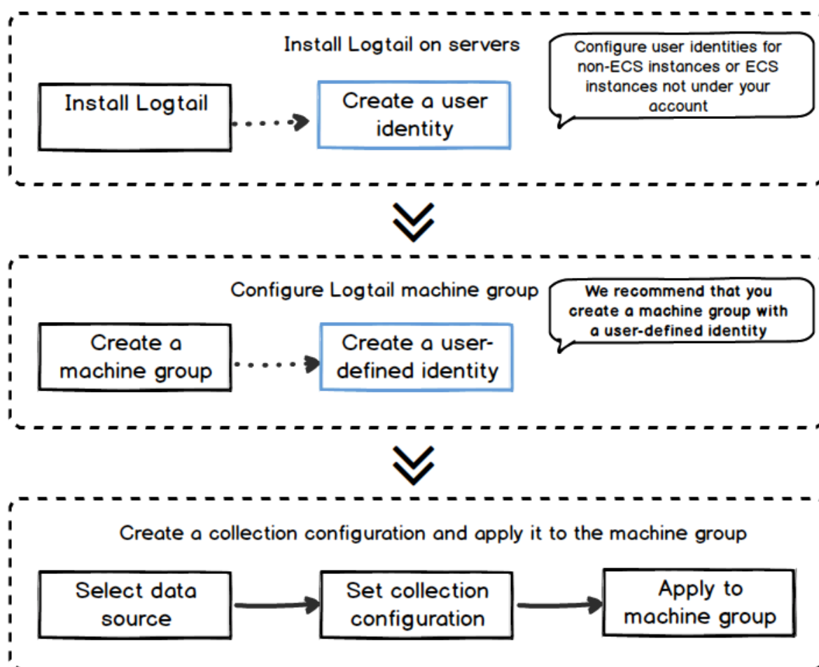
Figure 3-2: Configuration process
