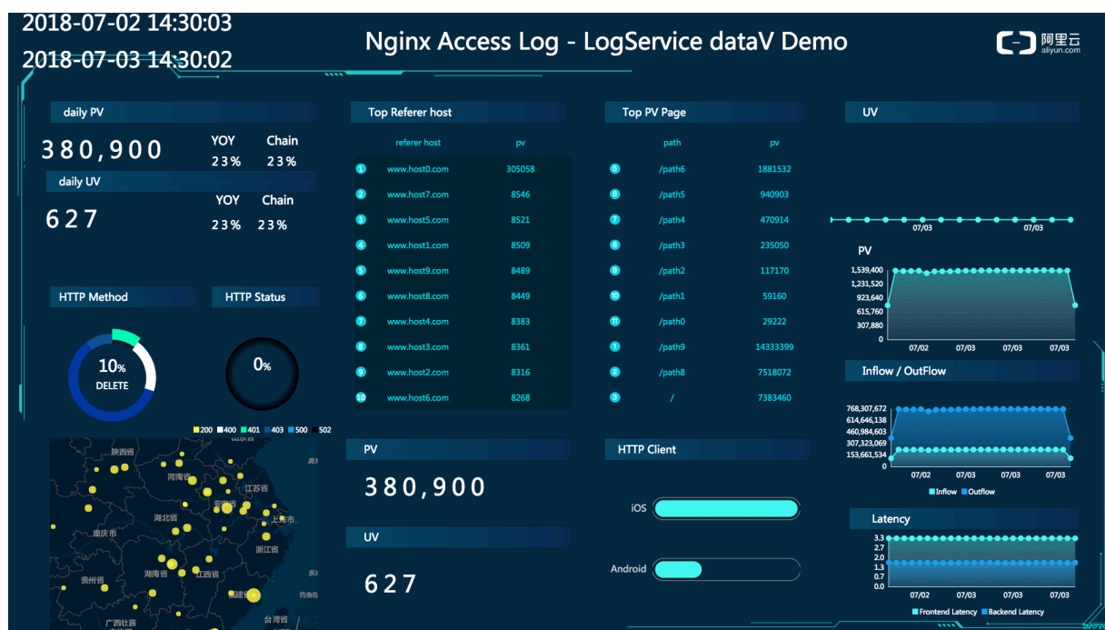
Figure 7-38: Real-Time Screen
