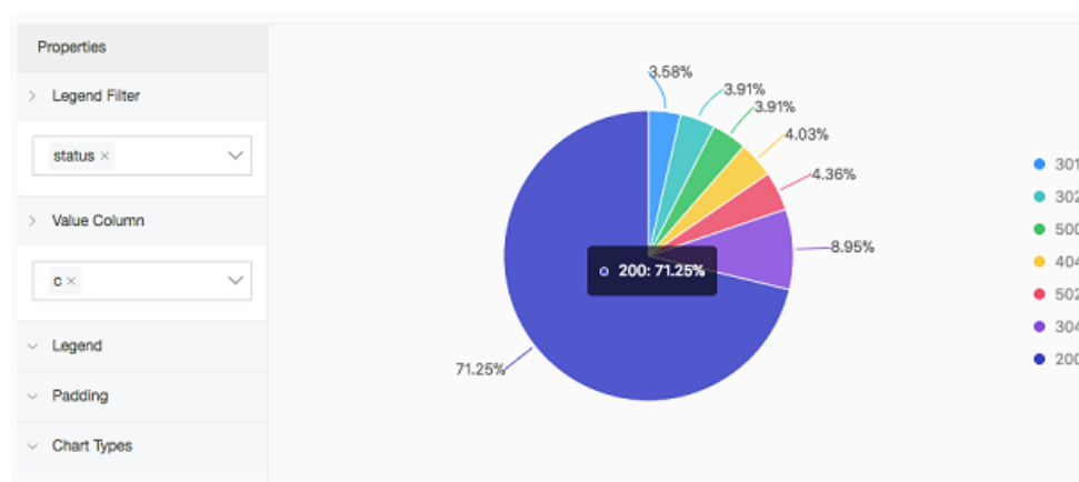
Figure 7-10: Pie chart
