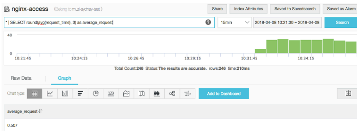
Figure 7-3: case 2
