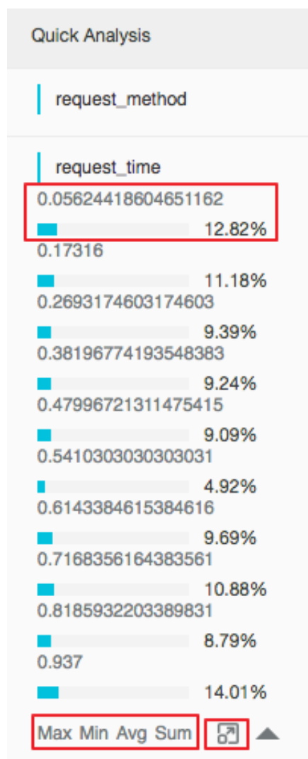
Figure 6-7: Request Distribution
