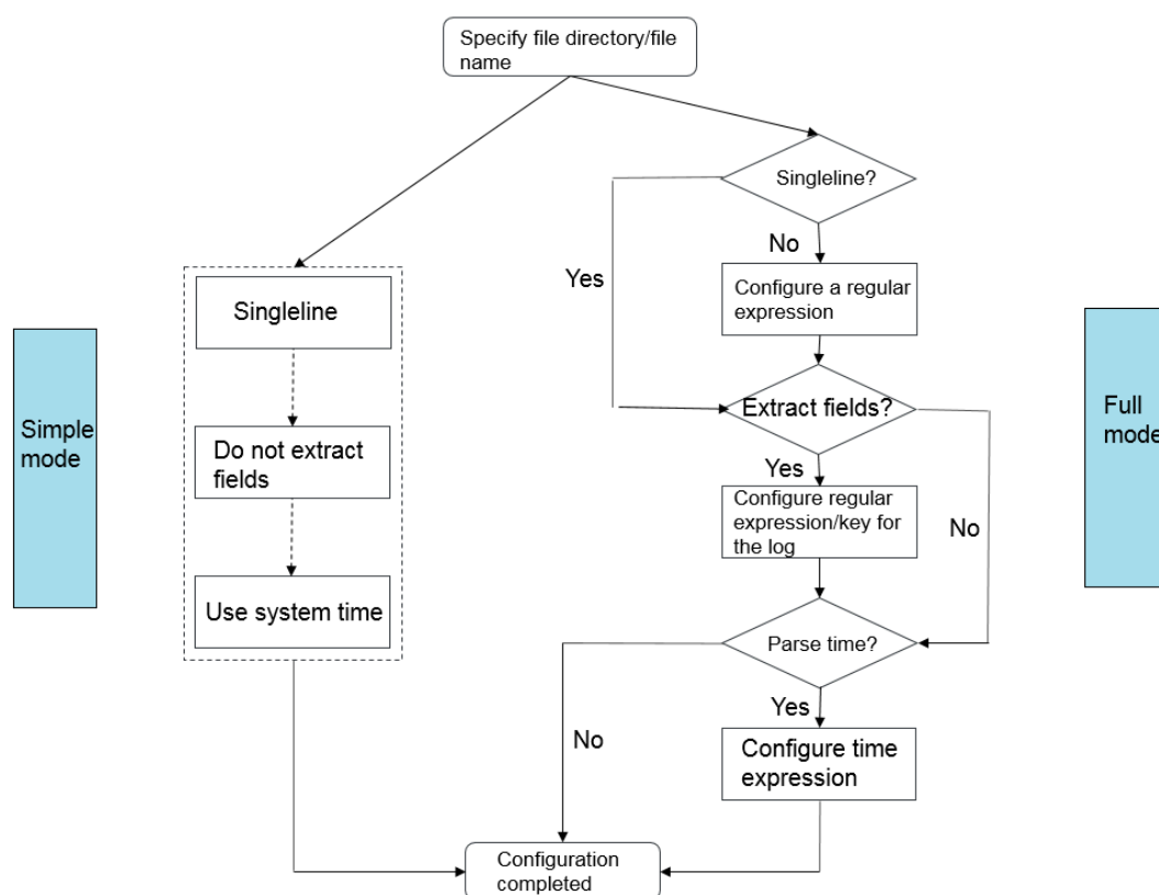
Figure 3-13: Log collection configuration process
