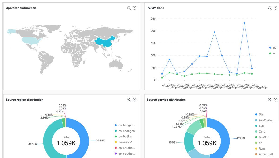
Figure 4-25: Trends of failed operations
