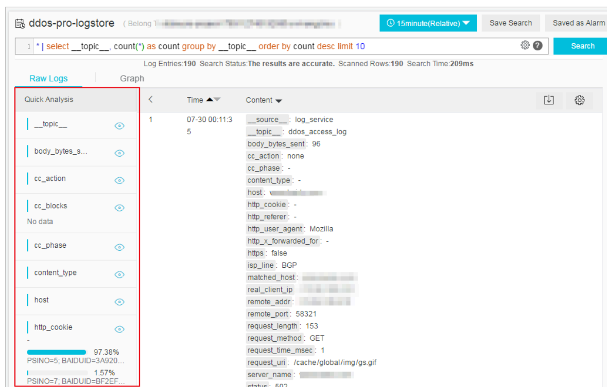
Figure 4-11: Quick analysis
