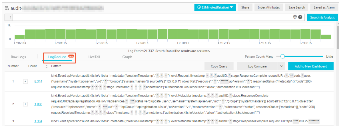
Figure 6-6: Result
