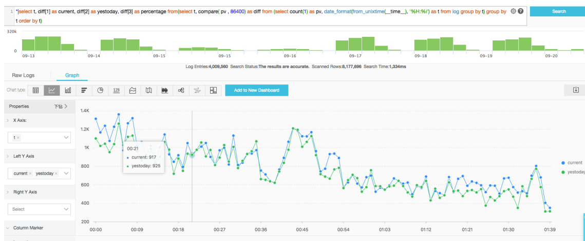
Figure 6-19: Line chart
