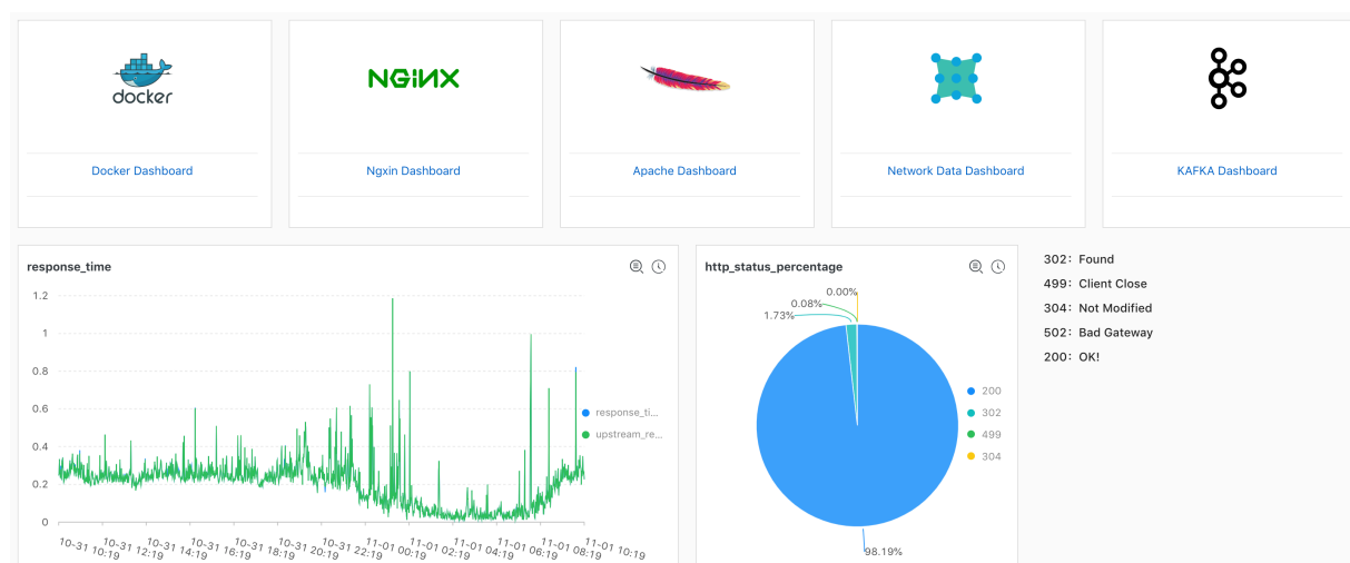
Figure 7-17: Scenarios
