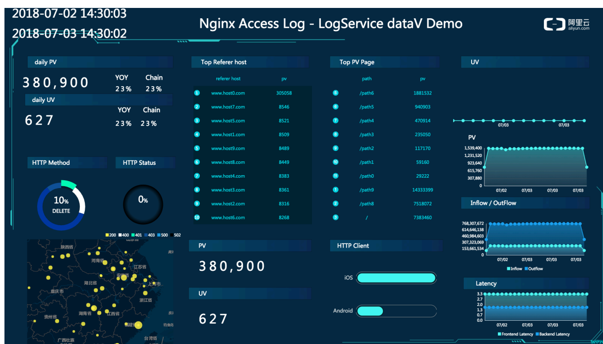
Figure 7-39: Real-Time Screen
