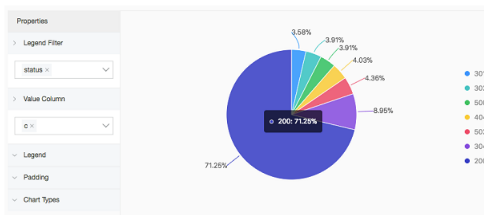
Figure 7-11: Pie chart
