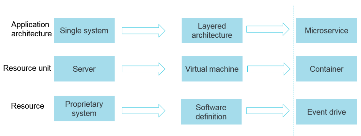
Figure 7-26: Architectural Evolution
