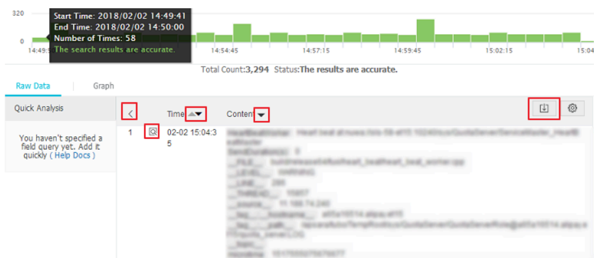
Figure 6-16: Raw logs
