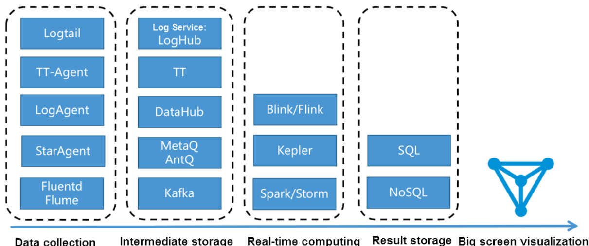
Figure 7-32: Related products
