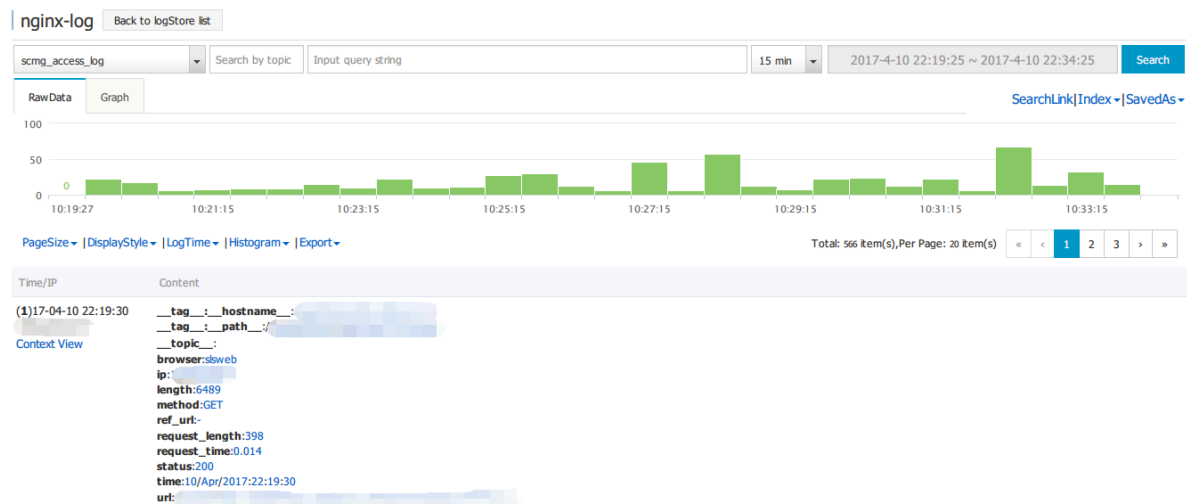
Figure 6-11: Query log
