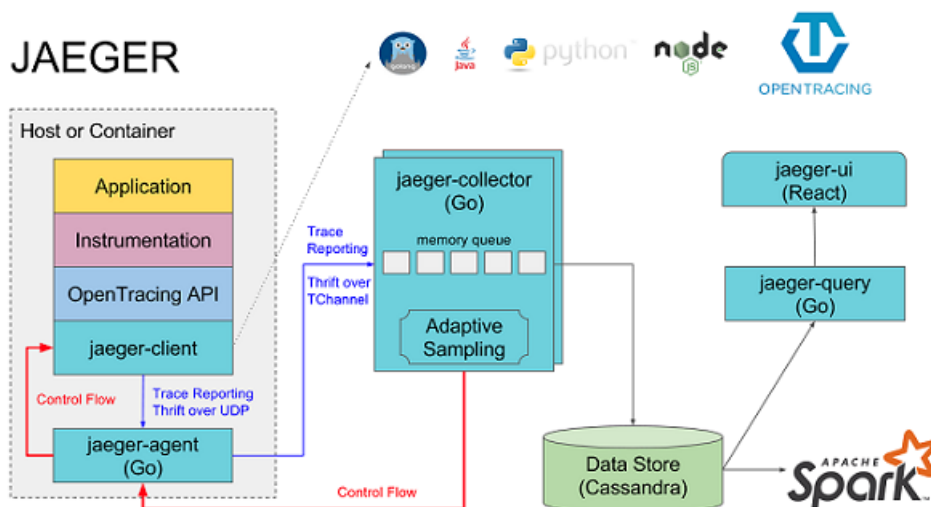
Figure 7-30: Architecture
