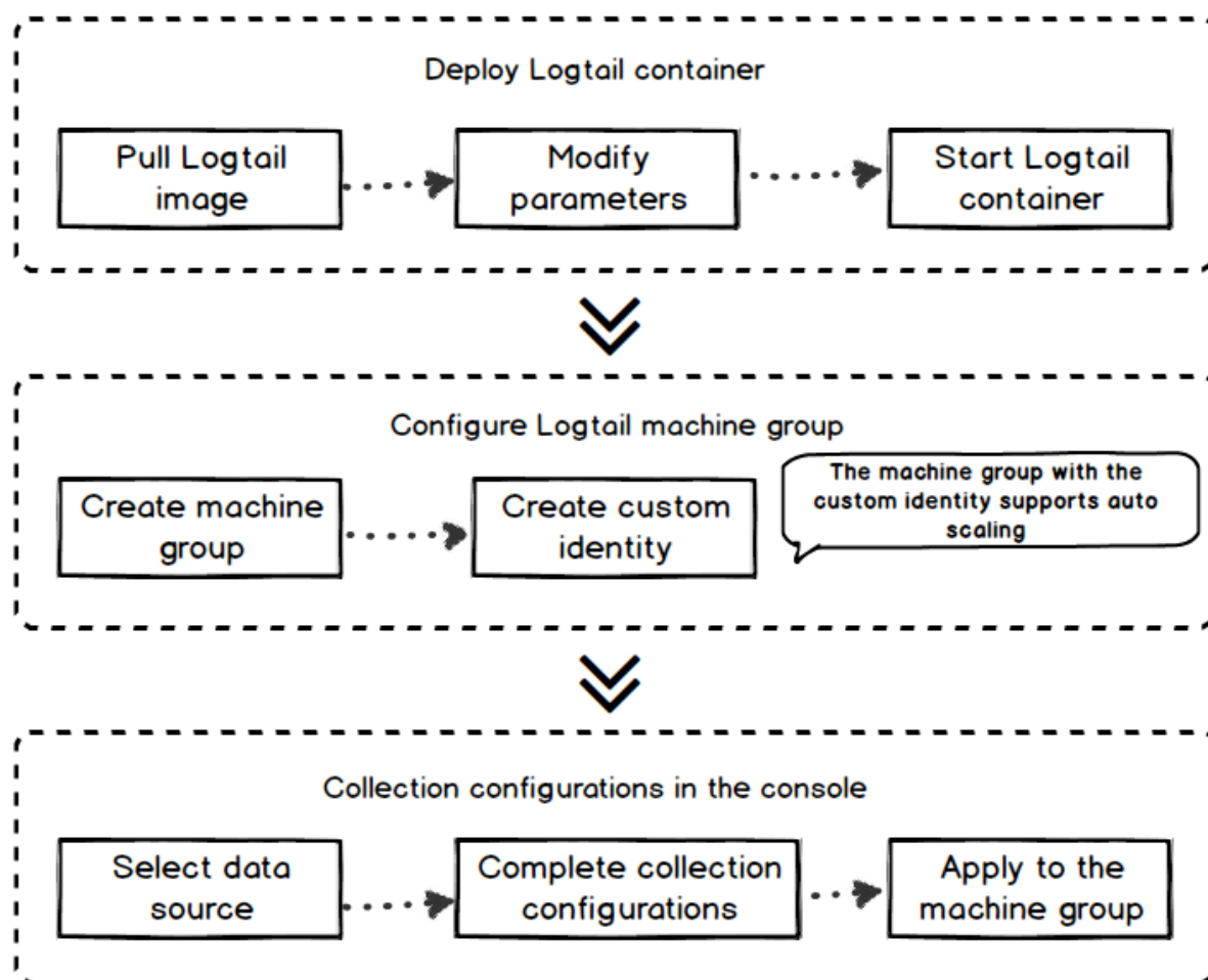
Figure 3-21: Configuration process
