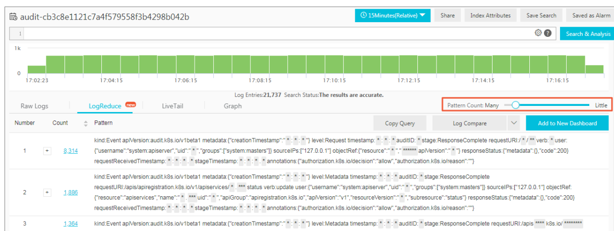
Figure 6-9: Adjust the log grouping tolerance
