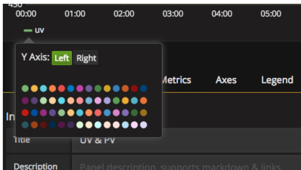
Figure 7-43: Y-axis display
