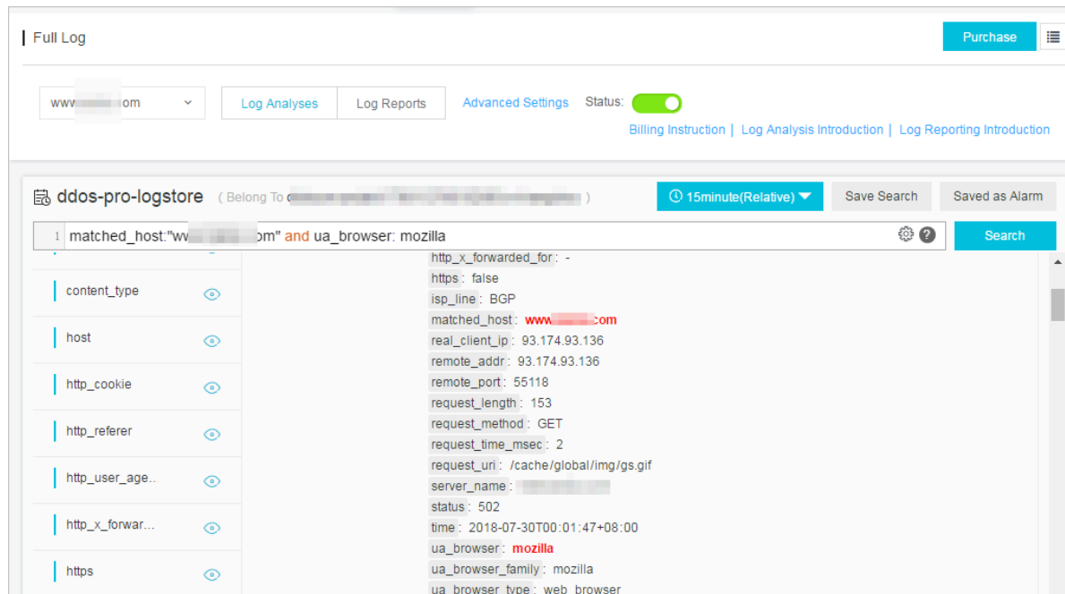
Figure 4-17: Log query
