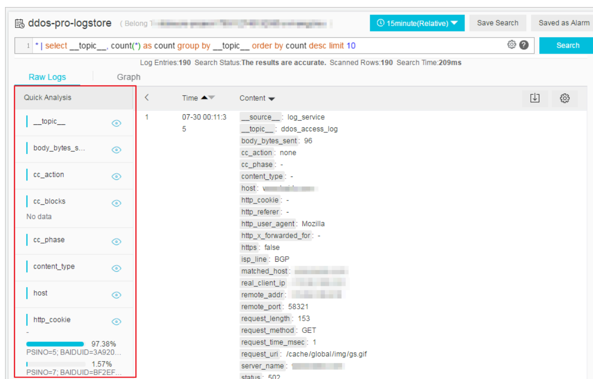
Figure 4-21: Quick analysis
