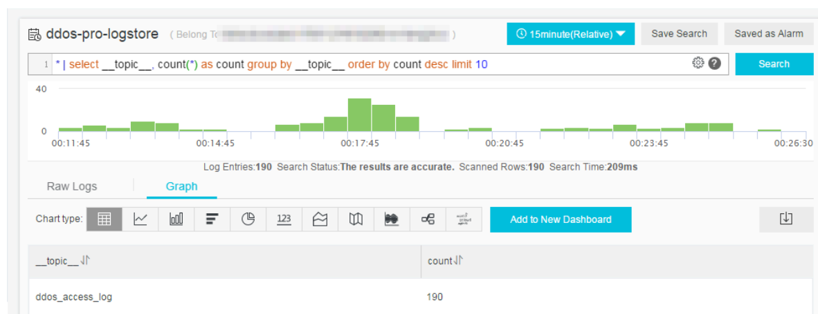
Figure 4-20: Chart
