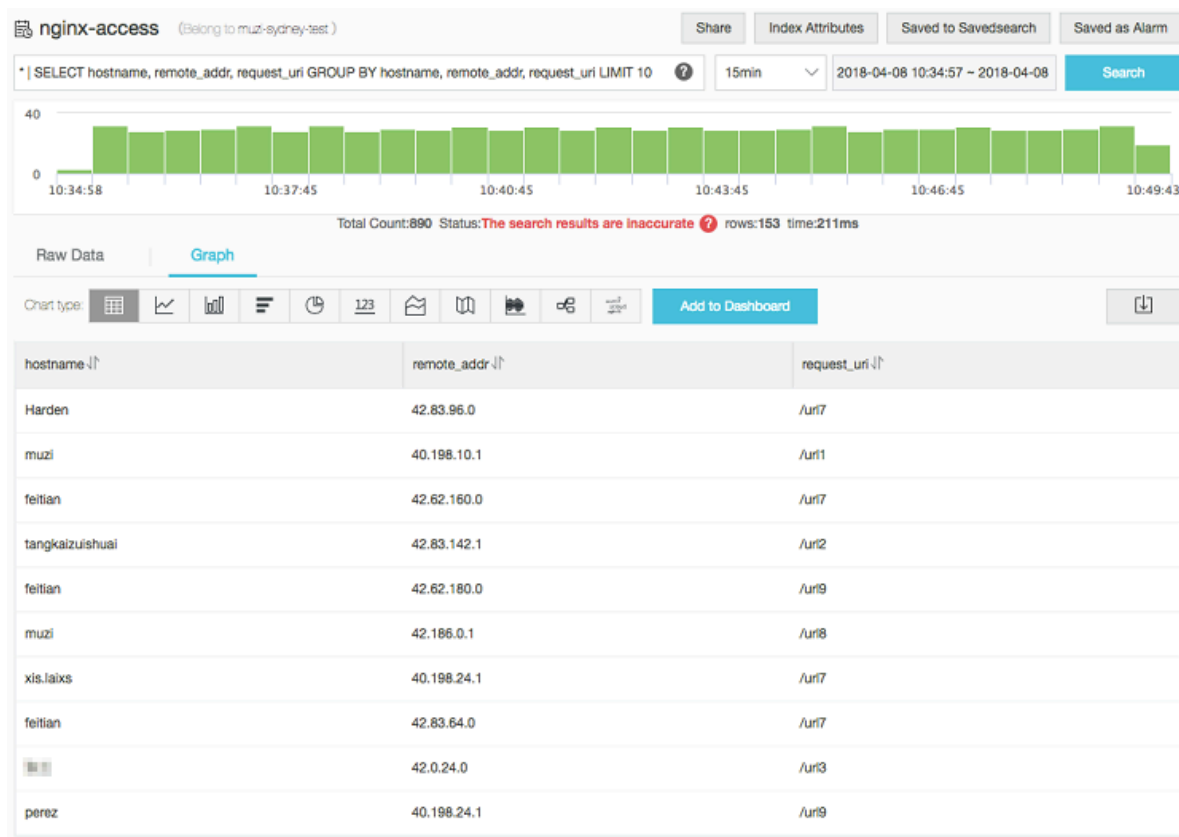
Figure 7-3: case 1
