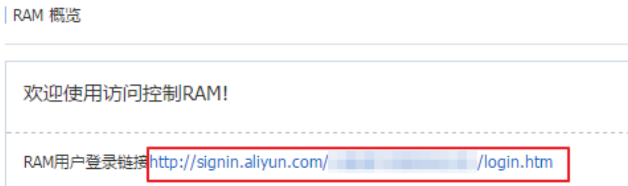
Figure 12-1: RAM user
