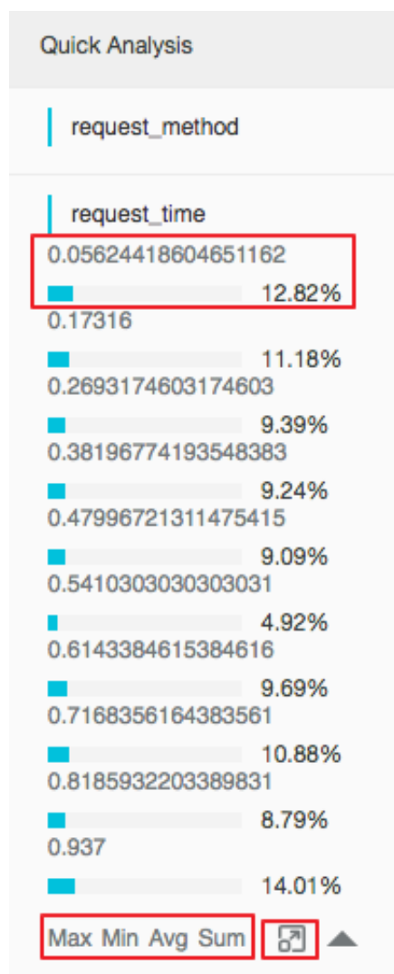
Figure 6-15: Request Distribution
