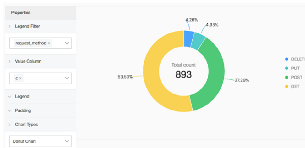
Figure 7-12: Cycle graph
