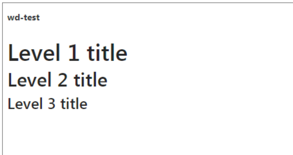
Figure 7-19: Title preview
