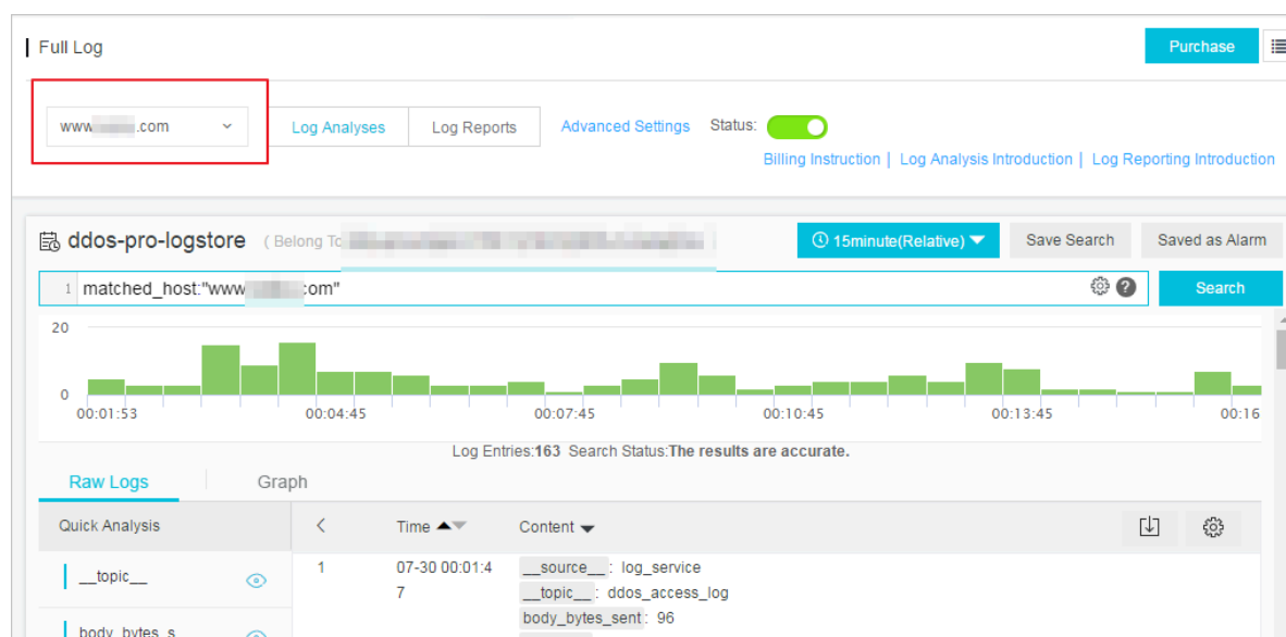
Figure 4-16: Analyze logs
