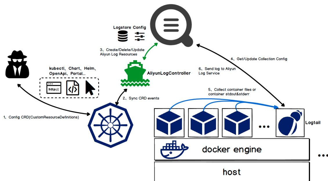
Figure 3-29: Implementation principles
