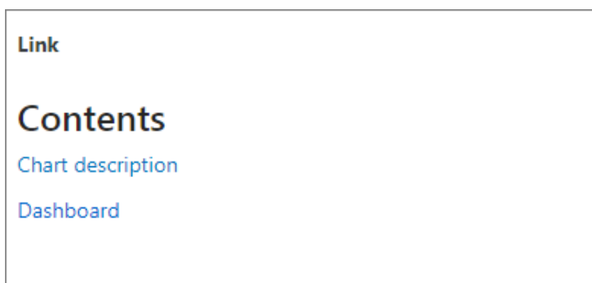
Figure 7-20: Link preview
