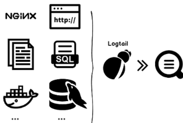
Figure 3-1: Function advantages
