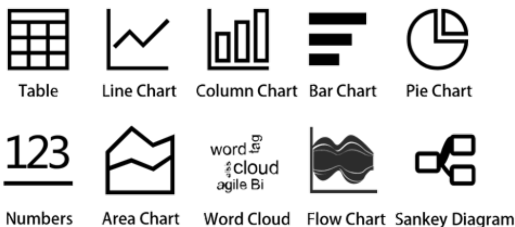
Figure 7-1: Graph type
