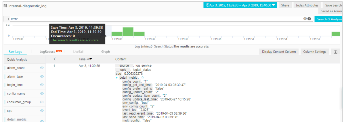
Figure 8-1: Query statement
